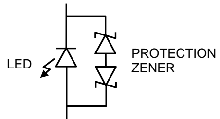
Equivalent Circuit
